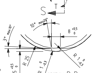
SECTION R-R
