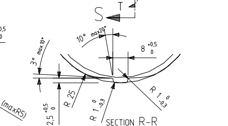
SECTION R-R
