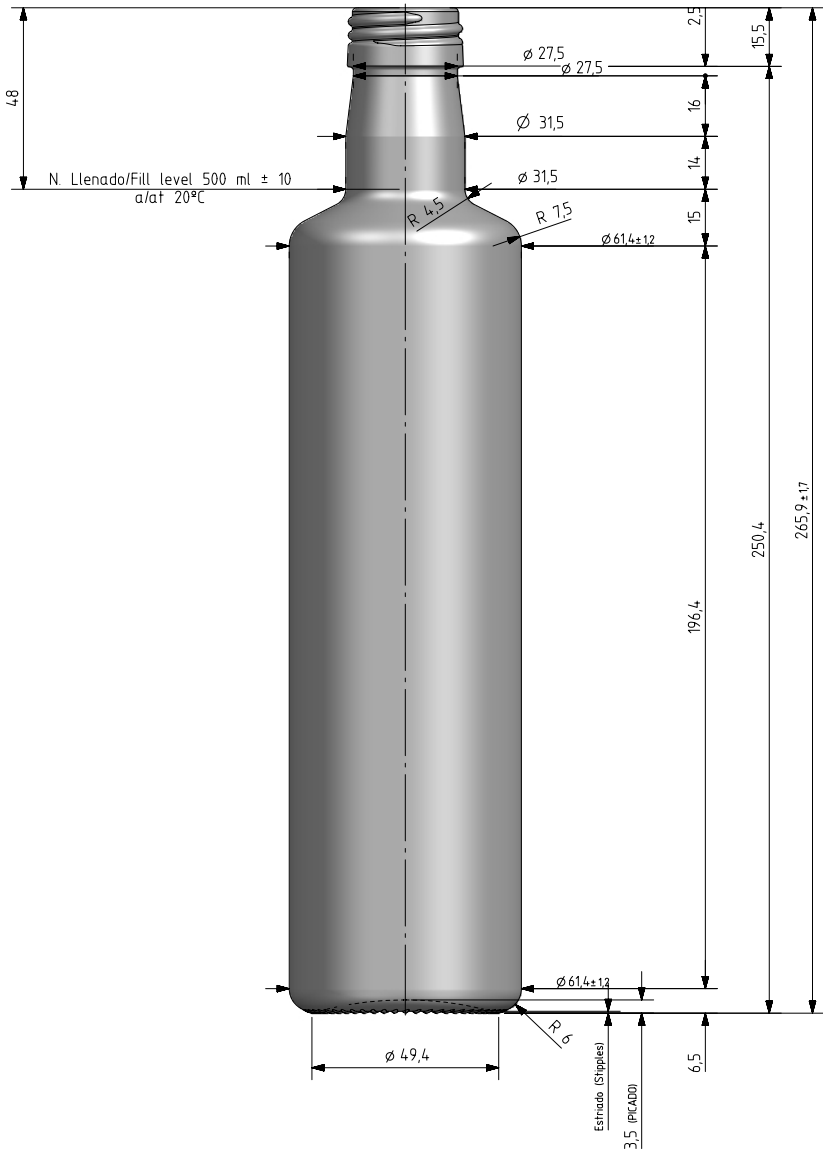
VISTA FRONTAL (FRONT VIEW)
