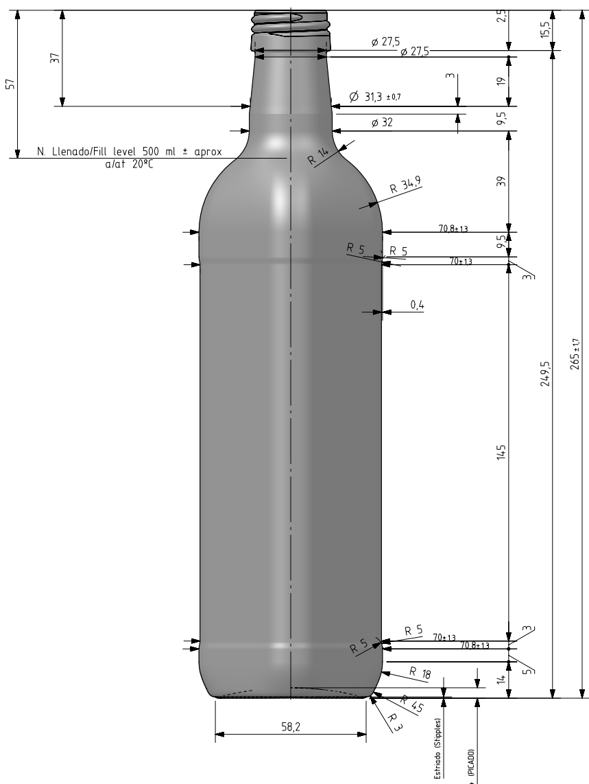
VISTA DIAGONAL (DIAGONAL VIEW)
